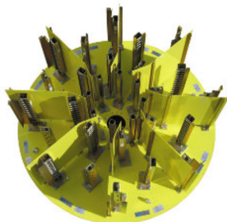
Turntable buffer
