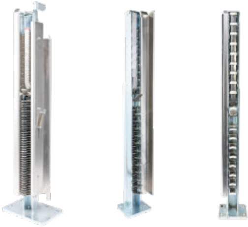
Stacking columns and part support
